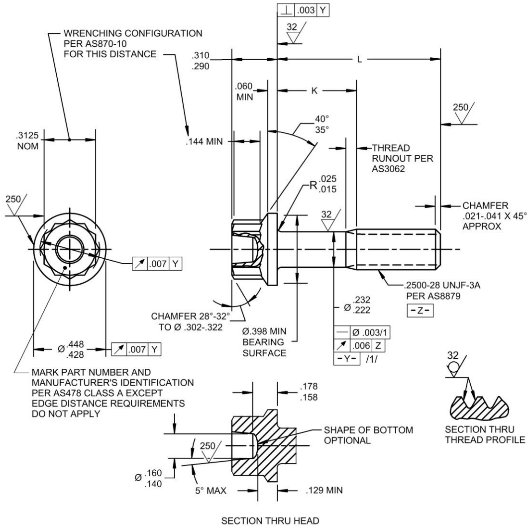
FIGURE 1 - BOLT
